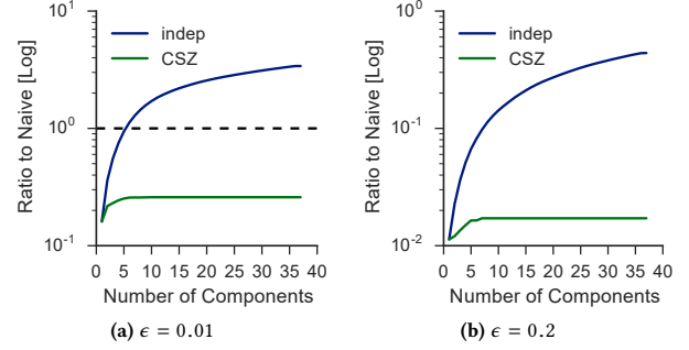
Figure 4: Communication cost for tracking increasing number of PCA scores (log scaled) for strict and relaxed error bounds. Independent tracking scales poorly: in both cases, the communication cost of indep grows sharply. For strict \epsilon = 0.01 indep quickly becomes worse than naive. The CSZ method scales much better: its cost grows slowly and becomes constant after the first few scores. In both cases, the cost of CSZ remains well below both naive and indep.
